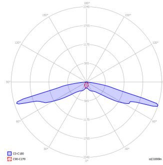
Corridor Beam
