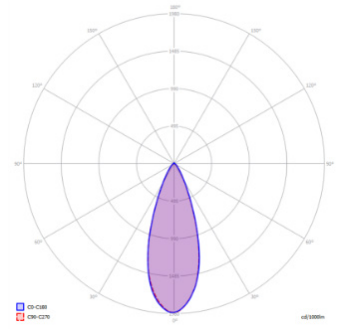
36° Beam Angle
