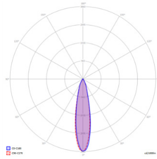
24° Beam Angle
